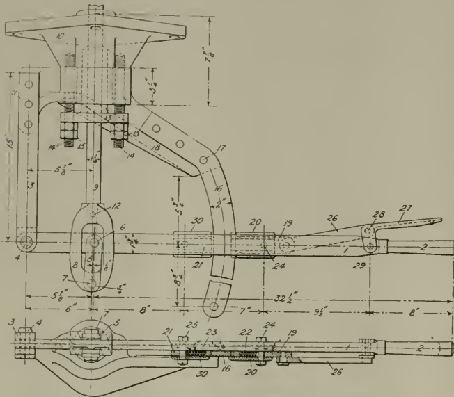
DETAILS OF THROTTLE LEVER AND ATTACHMENTS
